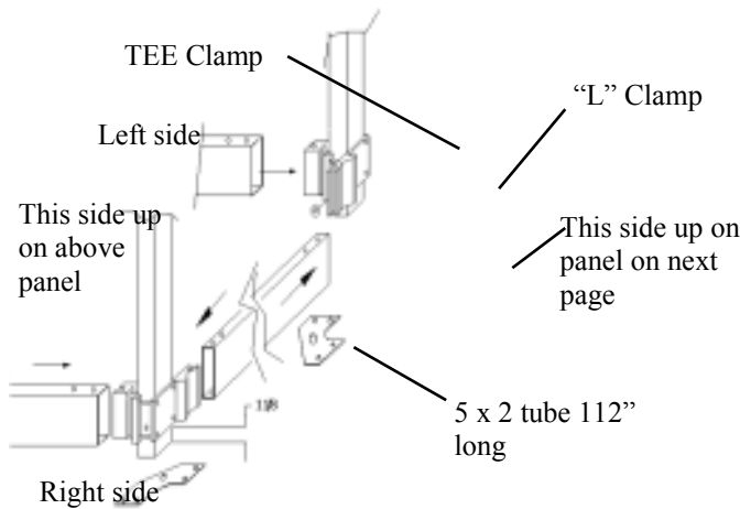
Drawing of lower side panel
