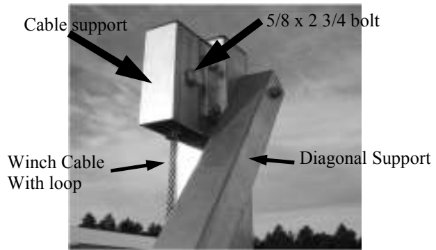
View of winch side, rear corner of hoist.
