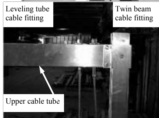
View of non winch column front
