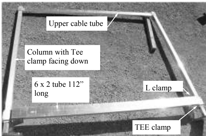
Left hand column
