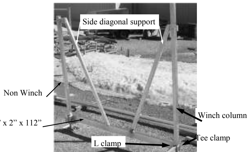
View of non winch side panel
